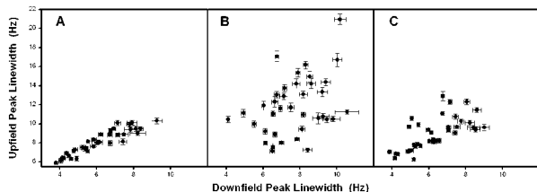
Figure 1. Upfield vs downfield line widths of (A) protein L alone, (B) protein L plus PM, and (C) protein L plus PM and 0.8 equiv of Tb 3+ .
